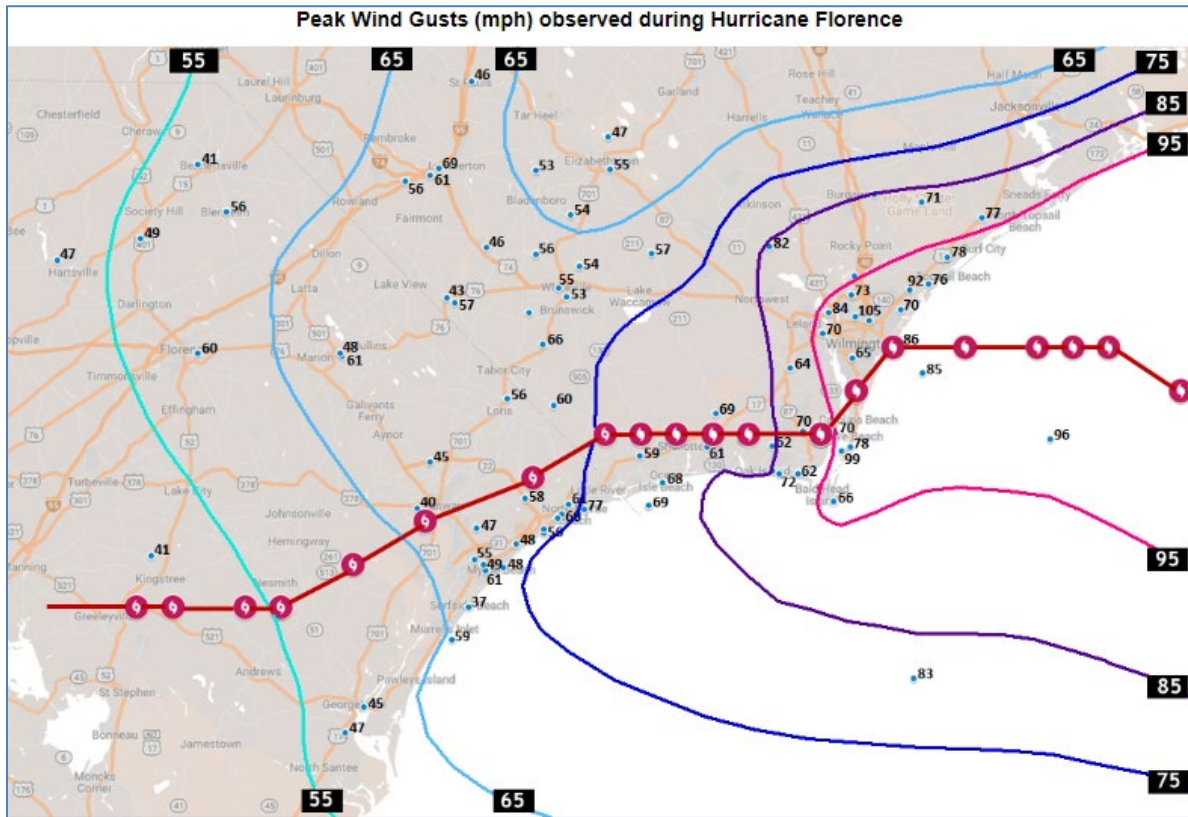
Figure 2 - Wind Gusts in MPH, September 14, 2018, Hurricane Florence (NWS)
